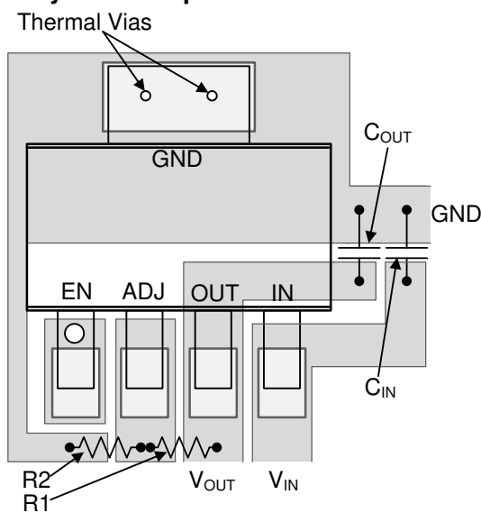
Figure 33. LP38692-ADJ SOT-223 Package
