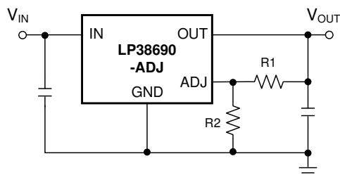
Simplified Schematic LP38690-ADJ
